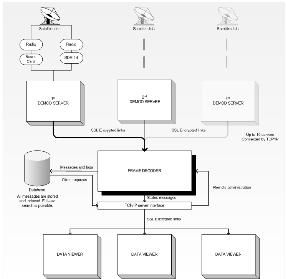
Block diagram of typical Inmarsat-C collection system
